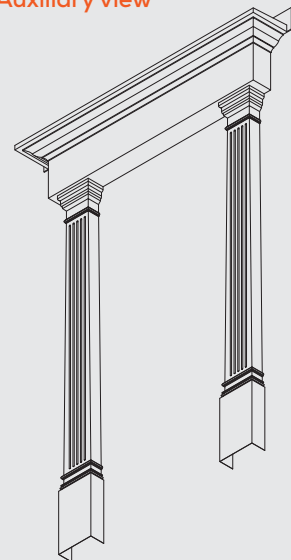
Auxiliary view
